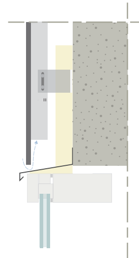
Figure 26: EQUITONE base detail Curtain Wall
