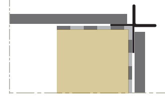
Figure 6: External Corner with trim Timber subframe
