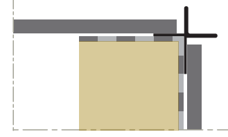
Figure 6: External Corner with trim Timber subframe
